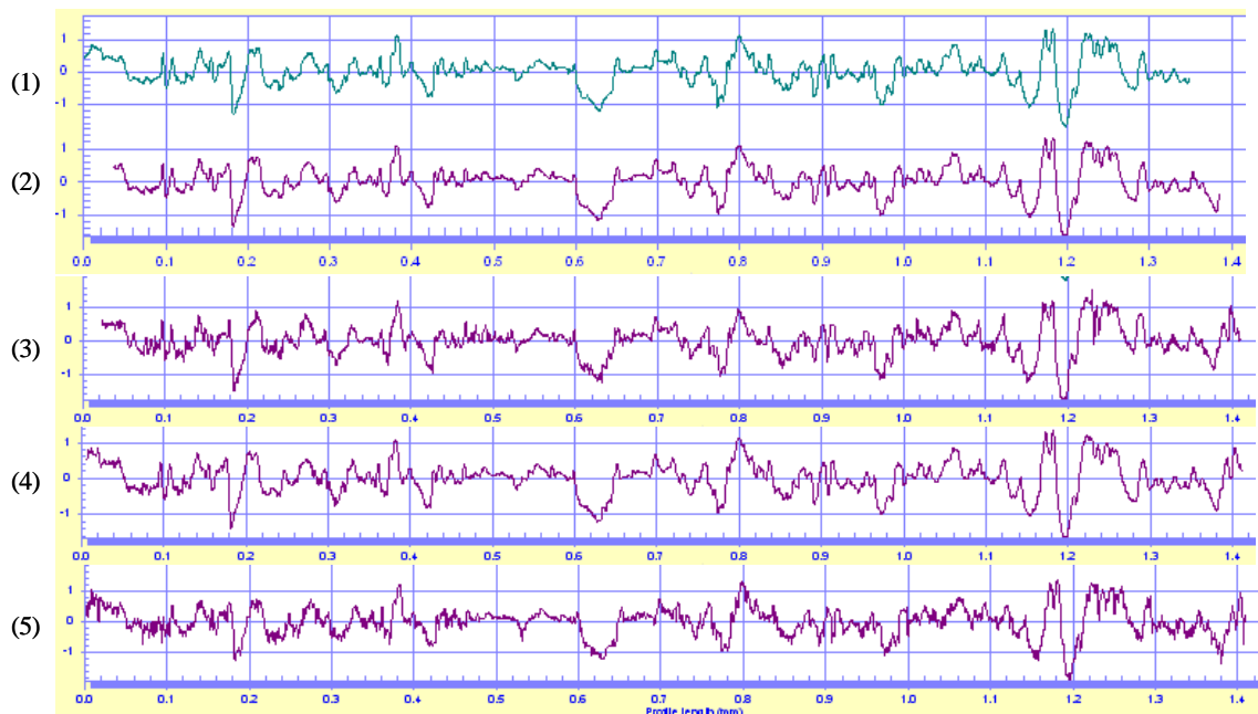
Fig. 3. The signature profiles of LEA 1 of SRM 2460-001 bullet were measured by four techniques (2 to 5) and correlated with the stylus profile of the virtual standard (1). Profile 2 was traced by a stylus instrument, CCF_{\max} = 99.6\% ; Profile 3 was traced by an interferometric microscope, CCF_{\max} = 92.1\% ; Profile 4 was traced by a Nipkow disk confocal microscope, CCF_{\max} = 99.0\% ; Profile 5 was traced by a laser scanning confocal microscope, CCF_{\max} = 95.3\% . The vertical scale covers \pm 1\ \mu\text{m} , the horizontal scale covers 0 - 1.4 mm.
