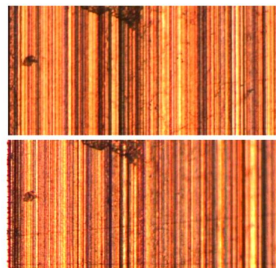
Fig. 2. Two images captured on the same area of the SRM 2460-001 bullet by the same microscope under different lighting directions. (Top) – Area aligned perpendicular to microscope optical axis, (Bottom) – The same area tilted by approximately 6°.
